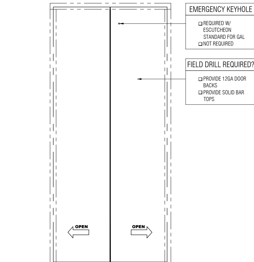
ELEVATION - CORRIDOR SIDE
